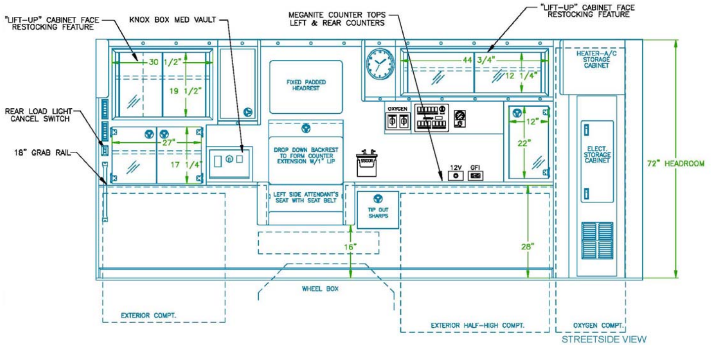
Streetside Layout
