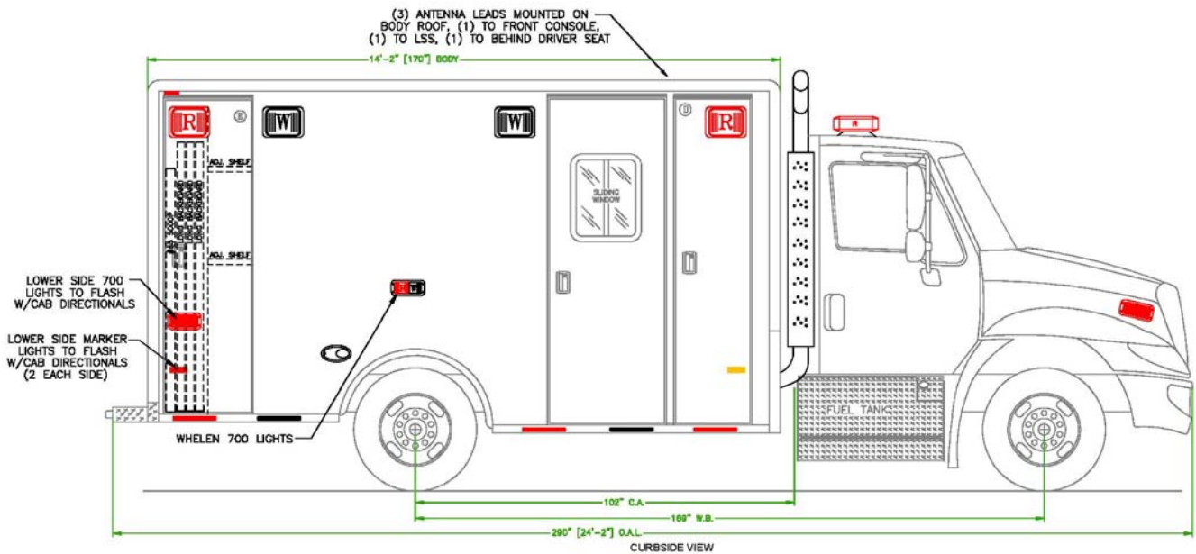
CURBSIDE VIEW
