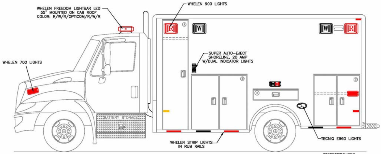
STREETSIDE VIEW
